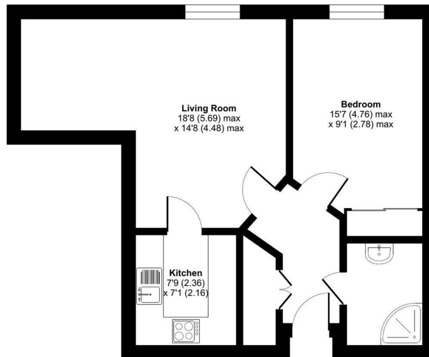
THIRD FLOOR
